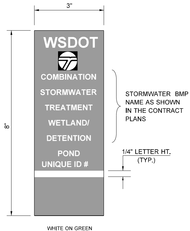
WSDOT STORMWATER BMP STICKER (FACING TRAFFIC) NTS
