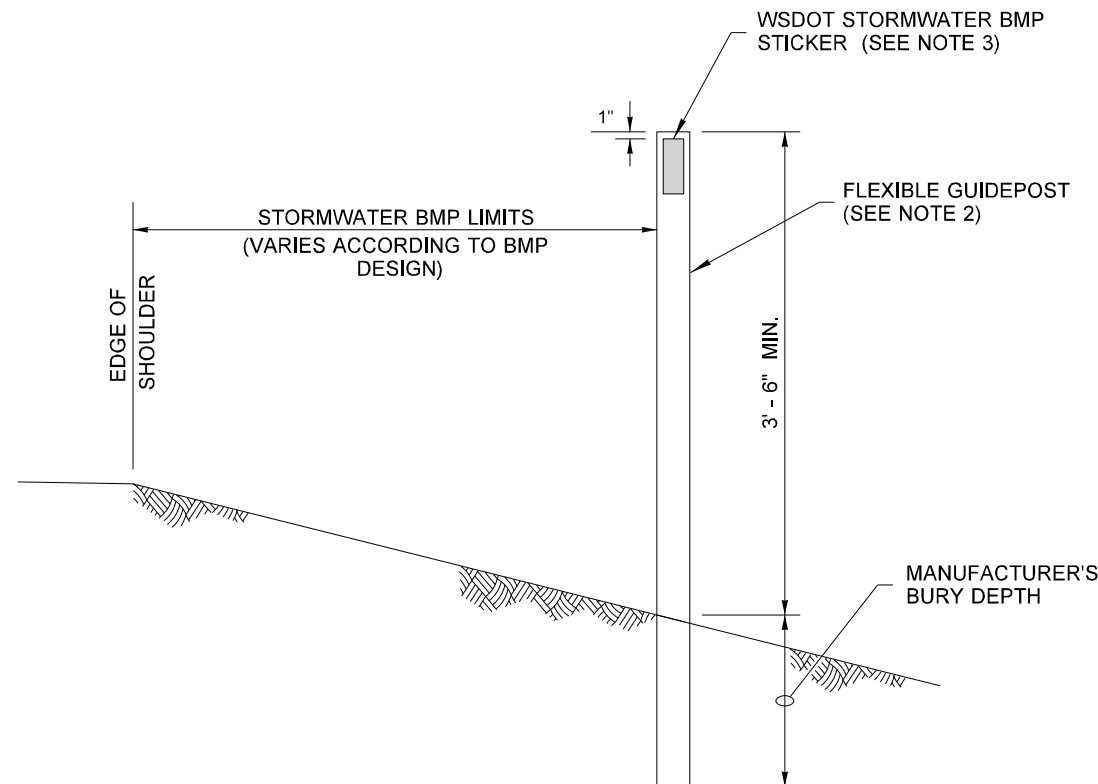
FLEXIBLE GUIDE POST DETAIL TYPICAL FOR ALL STORMWATER BMP GUIDE POSTS AS DETAILED ON THIS SHEET
